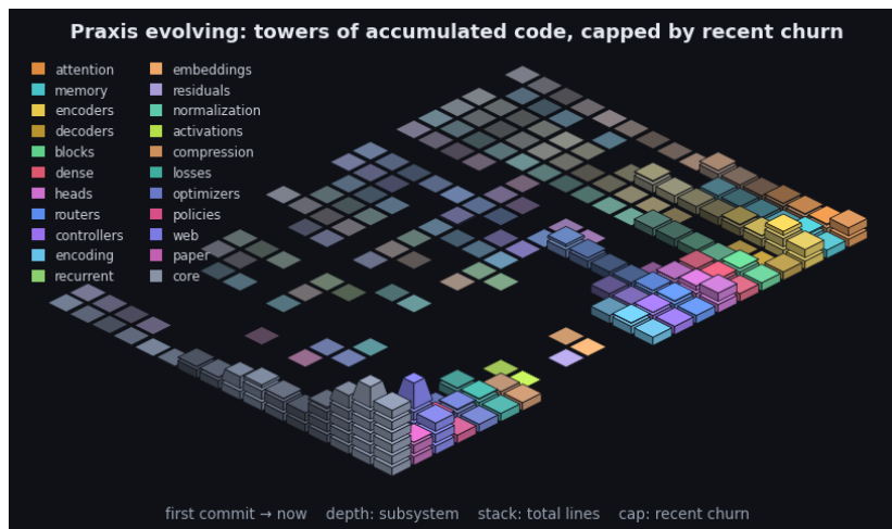
Figure 5: Praxis’s git history as an isometric terrain over the last 2358 commits. Each cell is one subsystem in one time window: a stack of base blocks for its accumulated size (total lines, recency-weighted) topped by a vivid cap for that window’s line churn - the standing codebase carrying the recent activity. Both are weighted by recency (the kernel the model applies to a sequence, turned on the repository): recent windows stack tall with bright caps while history thins toward the always-present prior - the low valley we roll into. Color fades from each subsystem’s hue toward a neutral prior into the past, banded in phased strata over a non-linear timescale. It is the bias/variance geometry read along the frequency axis (see the project notes): loud recent corrections over the quiet, ever-present base. By recency-weighted churn the current center of gravity is core, web, paper. The framework charts the hand that builds it.
