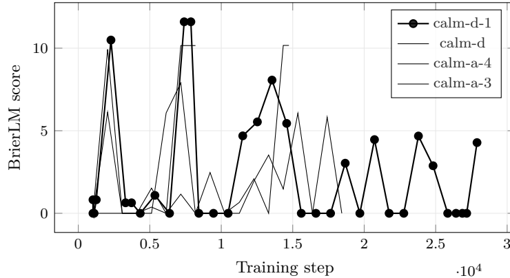
Figure 6: BrierLM across the 4 most recent experiments with comparable validation curves; the leading run ( calm-d-1 ) is drawn in bold. Generated from run logs - metrics that are not comparable across families (token loss vs. byte bits-per-byte vs. codec/CALM BrierLM) are excluded by construction, so the curves on this axis mean the same thing.
