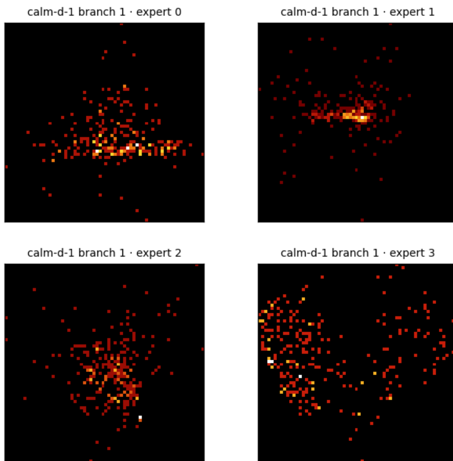
Figure 4: Center PCA density for the 4 crystal heads of calm-d-1 - a single multi-head model (prismatic4’s VEAR crystal bank), so these are that run’s own heads (branch 1 · expert 0, branch 1 · expert 1, branch 1 · expert 2, branch 1 · expert 3), not a cross-run mix. Each panel is the top-2 PCA projection of a head’s vocabulary centers, binned to a 64 \times 64 density grid (log color) - the same snapshot the dashboard renders live. The bank’s experts settle into structurally distinct geometries - the between-expert variance the router selects over.
