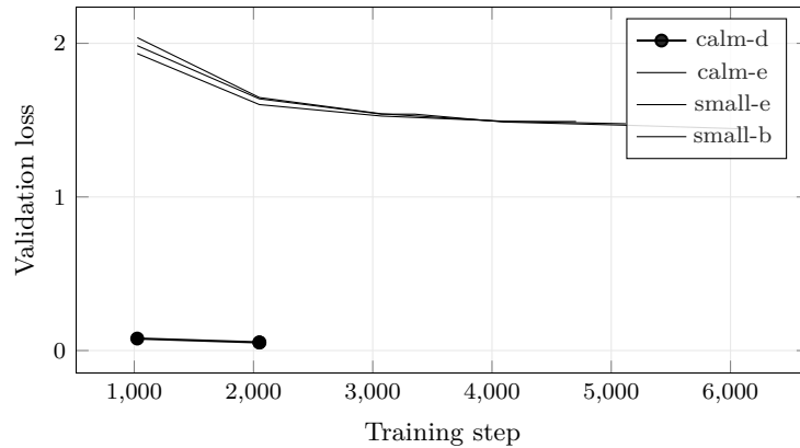
Figure 8: Validation Loss across the 4 most recent experiments with comparable validation curves; the leading run ( calm-d ) is drawn in bold. Generated from run logs - metrics that are not comparable across families (token loss vs. byte bits-per-byte vs. codec/CALM BrierLM) are excluded by construction, so the curves on this axis mean the same thing.
