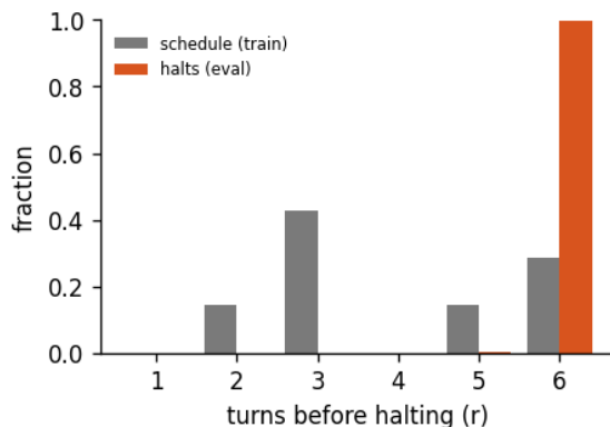
Figure 5: Halting distribution: the fraction of forward passes that stop after r turns, for the 6-turn recurrent loop of run calm-d, early-halt rate 0%, mean boundary KL 159. schedule is the random loop-count the model trains under; halts is where the KL gate actually stops at inference. A mass pinned at the maximum (KL never collapsing) is the honest signature of a model that has not yet learned to converge early - the decision is real, not yet decisive.
