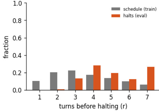
Figure 6: Halting distribution: the fraction of forward passes that stop after r turns, for the 7-turn recurrent loop of run abstractinator-b, early-halt rate 15%, mean boundary KL 0.255. schedule is the random loop-count the model trains under; halts is where the KL gate actually stops at inference. A mass pinned at the maximum (KL never collapsing) is the honest signature of a model that has not yet learned to converge early - the decision is real, not yet decisive.
