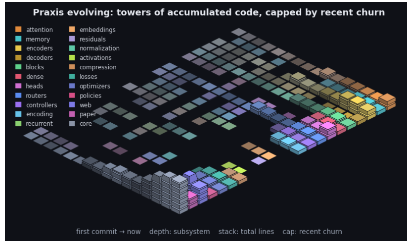
Figure 10: Praxis's git history as an isometric terrain over the last 2405 commits. Each cell is one subsystem in one time window: a stack of base blocks for its accumulated size (total lines, recency-weighted) topped by a vivid cap for that window's line churn - the standing codebase carrying the recent activity. Both are weighted by recency (the kernel the model applies to a sequence, turned on the repository): recent windows stack tall with bright caps while history thins toward the always-present prior - the low valley we roll into. Color fades from each subsystem's hue toward a neutral prior into the past, banded in phased strata over a non-linear timescale. It is the bias/variance geometry read along the frequency axis (see the project notes): loud recent corrections over the quiet, ever-present base. By recency-weighted churn the current center of gravity is core, web, paper. The framework charts the hand that builds it.
