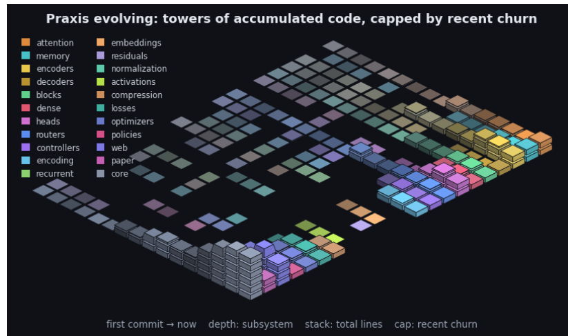
Figure 11: Praxis’s git history as an isometric terrain over the last 2426 commits. Each cell is one subsystem in one time window: a stack of base blocks for its accumulated size (total lines, recency-weighted) topped by a vivid cap for that window’s line churn - the standing codebase carrying the recent activity. Both are weighted by recency (the kernel the model applies to a sequence, turned on the repository): recent windows stack tall with bright caps while history thins toward the always-present prior - the low valley we roll into. Color fades from each subsystem’s hue toward a neutral prior into the past, banded in phased strata over a non-linear timescale. It is the bias/variance geometry read along the frequency axis (see the project notes): loud recent corrections over the quiet, ever-present base. By recency-weighted churn the current center of gravity is core, web, paper. The framework charts the hand that builds it.
