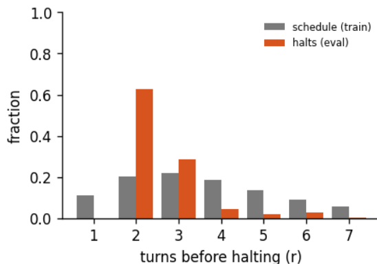
Figure 7: Halting distribution: the fraction of forward passes that stop after r turns, for the 7-turn recurrent loop of run abstractinator-c, early-halt rate 39%, mean boundary KL 0.471. schedule is the random loop-count the model trains under; halts is where the KL gate actually stops at inference. A mass pinned at the maximum (KL never collapsing) is the honest signature of a model that has not yet learned to converge early - the decision is real, not yet decisive.
