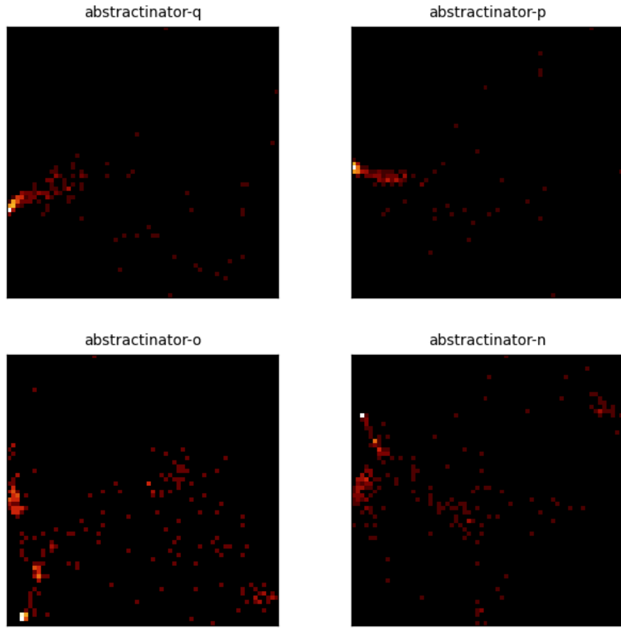
Figure 12: Center PCA density for the 4 most recent crystal-head runs (abstractinator-q, abstractinator-p, abstractinator-o, abstractinator-n). Each panel is the top-2 PCA projection of a head’s vocabulary centers, binned to a 64 \times 64 density grid (log color) - the same snapshot the dashboard renders live. Different runs settle into structurally different geometries, not noise.
