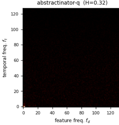
Figure 2: The static amplitude spectrum |a[f_t, f_d]| for abstractinator-q - the learned grid that, inverse-transformed through the frozen Weyl phases, becomes the bias field. This is the heatmap the text describes: energy that settles into a low-frequency band (small f_t, f_d ) is the corpus rhythm crystallizing, while a grid that stays uniform is a field still indistinguishable from noise. Hoyer concentration H = 0.32 quantifies it on the same [0, 1] scale the prose names (1 = a single cell, 0 = uniform), computed from this very tensor - the same value the dashboard logs live. The pink 1/f^\alpha prior lives in the frozen basis, not in these amplitudes, so the grid shown is exactly what the head exposes.
