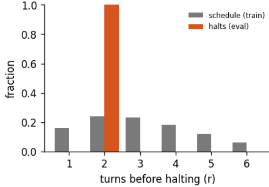
Figure 9: Halting distribution: the fraction of forward passes that stop after r turns, for the 6-turn recurrent loop of run abstractinator-q, early-halt rate 50%, mean boundary KL 0.965. schedule is the random loop-count the model trains under; halts is where the KL gate actually stops at inference. A mass pinned at the maximum (KL never collapsing) is the honest signature of a model that has not yet learned to converge early - the decision is real, not yet decisive.
