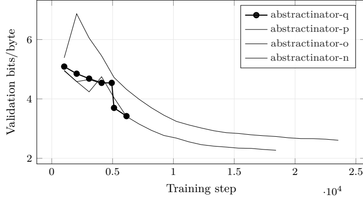
Figure 14: Bits per Byte across the 4 most recent experiments with comparable validation curves; the current experiment (abstractinator-q) is drawn in bold. Bold marks which run this build is reporting on , not which run scores best. The curves end wherever each run stopped, so they are at different points along their own training, and their endpoints are not a ranking. Generated from run logs - metrics that are not comparable across families (token loss vs. byte bits-per-byte vs. codec/CALM BrierLM) are excluded by construction, so the curves on this axis mean the same thing.
