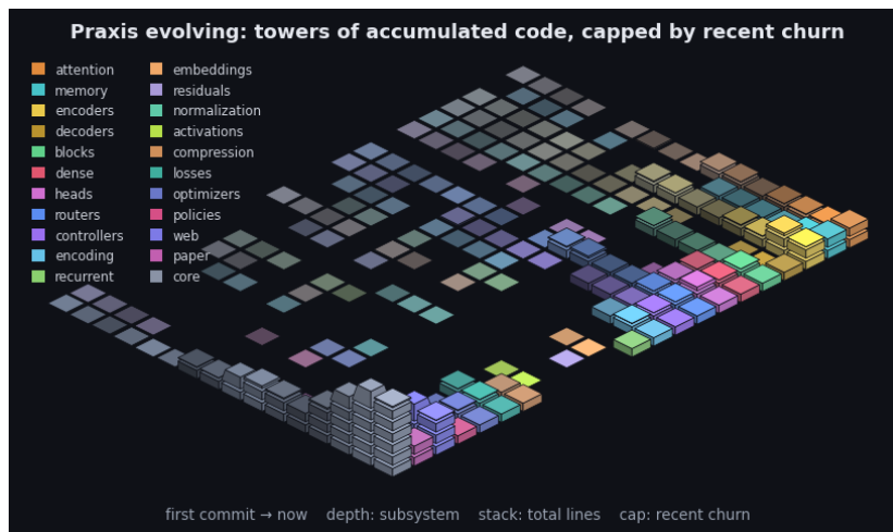
Figure 4: Praxis’s git history as an isometric terrain over the last 2269 commits. Each cell is one subsystem in one time window: a stack of base blocks for its accumulated size (total lines, recency-weighted) topped by a vivid cap for that window’s line churn - the standing codebase carrying the recent activity. Both are weighted by recency (the kernel the model applies to a sequence, turned on the repository): recent windows stack tall with bright caps while history thins toward the always-present prior - the low valley we roll into. Color fades from each subsystem’s hue toward a neutral prior into the past, banded in phased strata over a non-linear timescale. It is the bias/variance geometry read along the frequency axis (see the project notes): loud recent corrections over the quiet, ever-present base. By recency-weighted churn the current center of gravity is core, web, encoders. The framework charts the hand that builds it.
