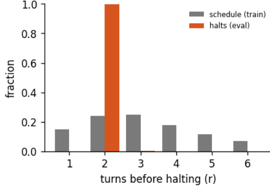
Figure 9: Halting distribution: the fraction of forward passes that stop after r turns, for the 6-turn recurrent loop of run abstractinator-p, early-halt rate 50%, mean boundary KL 1.53. schedule is the random loop-count the model trains under; halts is where the KL gate actually stops at inference. A mass pinned at the maximum (KL never collapsing) is the honest signature of a model that has not yet learned to converge early - the decision is real, not yet decisive.
