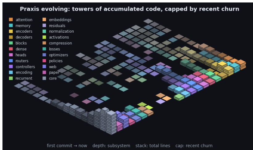
Figure 4: Praxis’s git history as an isometric terrain over the last 2268 commits. Each cell is one subsystem in one time window: a stack of base blocks for its accumulated size (total lines, recency-weighted) topped by a vivid cap for that window’s line churn - the standing codebase carrying the recent activity. Both are weighted by recency (the kernel the model applies to a sequence, turned on the repository): recent windows stack tall with bright caps while history thins toward the always-present prior - the low valley we roll into. Color fades from each subsystem’s hue toward a neutral prior into the past, banded in phased strata over a non-linear timescale. It is the bias/variance geometry read along the frequency axis (see the project notes): loud recent corrections over the quiet, ever-present base. By recency-weighted churn the current center of gravity is core, web, encoders. The framework charts the hand that builds it.
