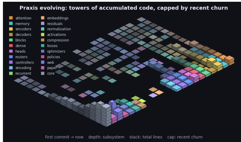
Figure 10: Praxis's git history as an isometric terrain over the last 2402 commits. Each cell is one subsystem in one time window: a stack of base blocks for its accumulated size (total lines, recency-weighted) topped by a vivid cap for that window's line churn - the standing codebase carrying the recent activity. Both are weighted by recency (the kernel the model applies to a sequence, turned on the repository): recent windows stack tall with bright caps while history thins toward the always-present prior - the low valley we roll into. Color fades from each subsystem's hue toward a neutral prior into the past, banded in phased strata over a non-linear timescale. It is the bias/variance geometry read along the frequency axis (see the project notes): loud recent corrections over the quiet, ever-present base. By recency-weighted churn the current center of gravity is core, web, paper. The framework charts the hand that builds it.
