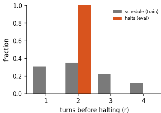
Figure 6: Halting distribution: the fraction of forward passes that stop after r turns, for the 4-turn recurrent loop of run abstractinator-a, early-halt rate 50%, mean boundary KL 0.391. schedule is the random loop-count the model trains under; halts is where the KL gate actually stops at inference. A mass pinned at the maximum (KL never collapsing) is the honest signature of a model that has not yet learned to converge early - the decision is real, not yet decisive.
