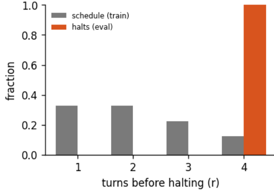
Figure 2: Halting distribution: the fraction of forward passes that stop after r turns, for the 4-turn recurrent loop of run calm-e, early-halt rate 0%, mean boundary KL 12.6. schedule is the random loop-count the model trains under; halts is where the KL gate actually stops at inference. A mass pinned at the maximum (KL never collapsing) is the honest signature of a model that has not yet learned to converge early - the decision is real, not yet decisive.
