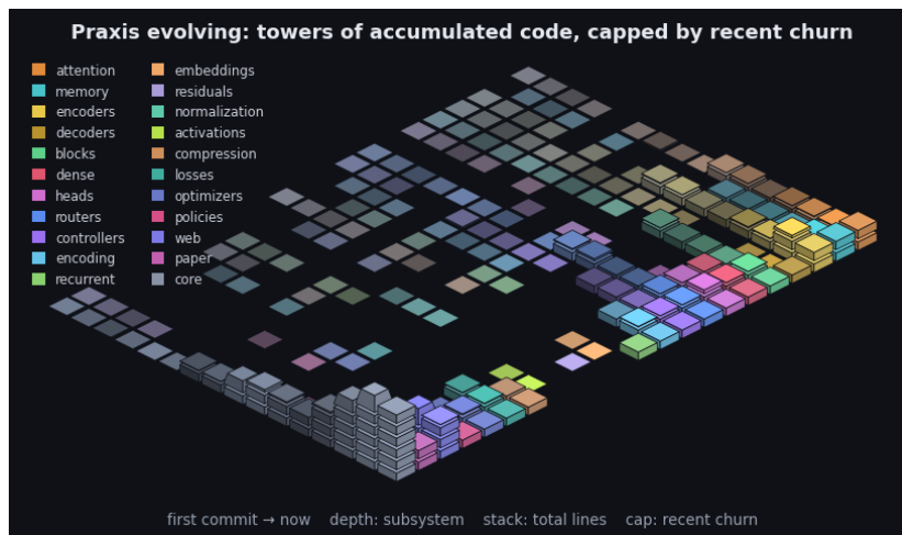
Figure 4: Praxis’s git history as an isometric terrain over the last 2260 commits. Each cell is one subsystem in one time window: a stack of base blocks for its accumulated size (total lines, recency-weighted) topped by a vivid cap for that window’s line churn - the standing codebase carrying the recent activity. Both are weighted by recency (the kernel the model applies to a sequence, turned on the repository): recent windows stack tall with bright caps while history thins toward the always-present prior - the low valley we roll into. Color fades from each subsystem’s hue toward a neutral prior into the past, banded in phased strata over a non-linear timescale. It is the bias/variance geometry read along the frequency axis (see the project notes): loud recent corrections over the quiet, ever-present base. By recency-weighted churn the current center of gravity is core, web, encoders. The framework charts the hand that builds it.
