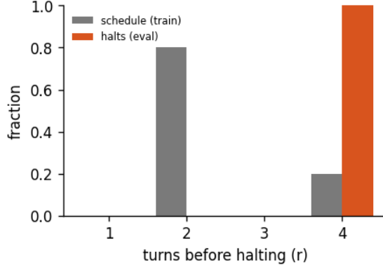
Figure 4: Halting distribution: the fraction of forward passes that stop after r turns, for the 4-turn recurrent loop of run calm-a, early-halt rate 0%, mean boundary KL 0.69. schedule is the random loop-count the model trains under; halts is where the KL gate actually stops at inference. A mass pinned at the maximum (KL never collapsing) is the honest signature of a model that has not yet learned to converge early - the decision is real, not yet decisive.
