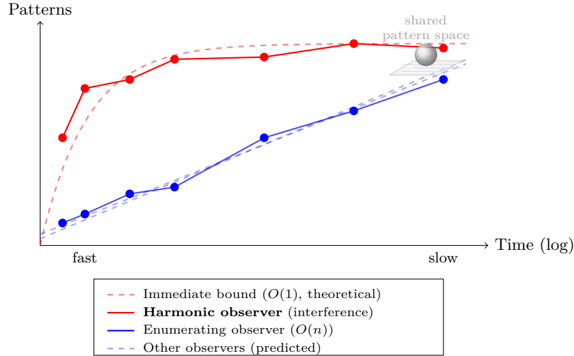
Figure 8: Schematic, not measured. The same convergence as Figure 6, read in the time domain rather than the resource domain. Different observers reach the same shared pattern space (the sphere over the plane, top right) along different temporal complexities: a harmonic observer composes by interference and has near-immediate, O(1) -like access (red, tracking the theoretical bound); an enumerating observer accumulates the same patterns one at a time, O(n) (blue), and other architectures (dashed) sit between. All converge asymptotically - the destination is shared, and it is the path to it, set by architecture, that differs. This is the intuitive companion to the cost figure, restored from an earlier draft and redrawn as the schematic it always was rather than the measurement it was once dressed as.
