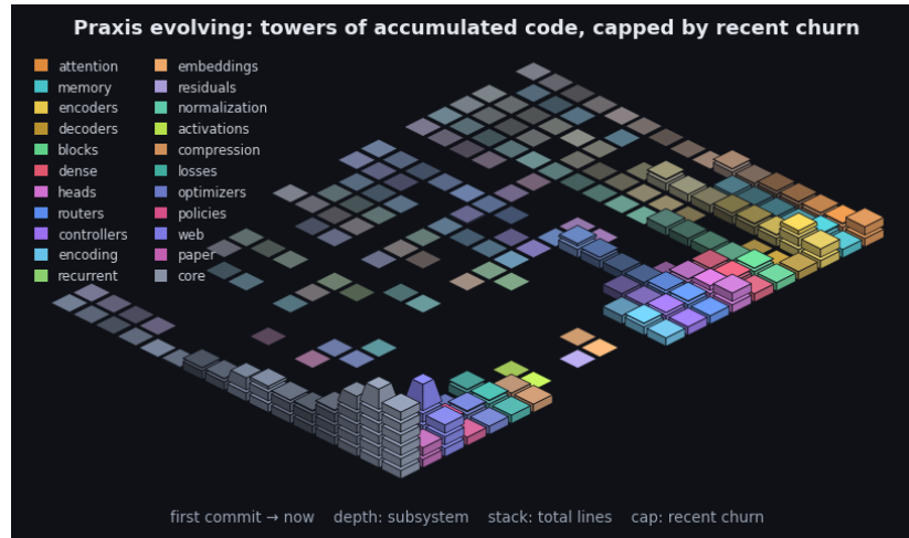
Figure 10: Praxis's git history as an isometric terrain over the last 2379 commits. Each cell is one subsystem in one time window: a stack of base blocks for its accumulated size (total lines, recency-weighted) topped by a vivid cap for that window's line churn - the standing codebase carrying the recent activity. Both are weighted by recency (the kernel the model applies to a sequence, turned on the repository): recent windows stack tall with bright caps while history thins toward the always-present prior - the low valley we roll into. Color fades from each subsystem's hue toward a neutral prior into the past, banded in phased strata over a non-linear timescale. It is the bias/variance geometry read along the frequency axis (see the project notes): loud recent corrections over the quiet, ever-present base. By recency-weighted churn the current center of gravity is core, web, paper. The framework charts the hand that builds it.
