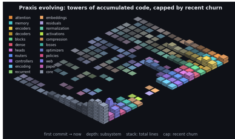
Figure 10: Praxis's git history as an isometric terrain over the last 2401 commits. Each cell is one subsystem in one time window: a stack of base blocks for its accumulated size (total lines, recency-weighted) topped by a vivid cap for that window's line churn - the standing codebase carrying the recent activity. Both are weighted by recency (the kernel the model applies to a sequence, turned on the repository): recent windows stack tall with bright caps while history thins toward the always-present prior - the low valley we roll into. Color fades from each subsystem's hue toward a neutral prior into the past, banded in phased strata over a non-linear timescale. It is the bias/variance geometry read along the frequency axis (see the project notes): loud recent corrections over the quiet, ever-present base. By recency-weighted churn the current center of gravity is core, web, paper. The framework charts the hand that builds it.
