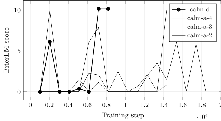
Figure 11: BrierLM across the 4 most recent experiments with comparable validation curves; the leading run (calm-d) is drawn in bold. Generated from run logs - metrics that are not comparable across families (token loss vs. byte bits-per-byte vs. codec/CALM BrierLM) are excluded by construction, so the curves on this axis mean the same thing.
