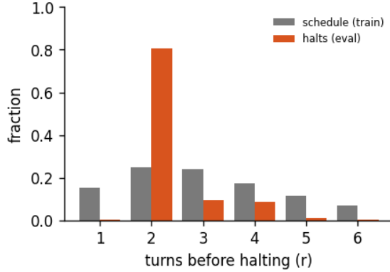
Figure 8: Halting distribution: the fraction of forward passes that stop after r turns, for the 6-turn recurrent loop of run abstractinator-f, early-halt rate 43%, mean boundary KL 1.03. schedule is the random loop-count the model trains under; halts is where the KL gate actually stops at inference. A mass pinned at the maximum (KL never collapsing) is the honest signature of a model that has not yet learned to converge early - the decision is real, not yet decisive.
