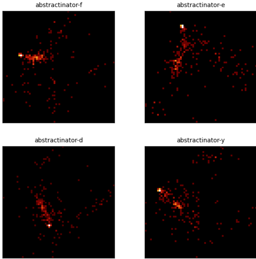
Figure 11: Center PCA density for the 4 most recent crystal-head runs ( abstractinator-f , abstractinator-e , abstractinator-d , abstractinator-y ). Each panel is the top-2 PCA projection of a head's vocabulary centers, binned to a 64 \times 64 density grid (log color) - the same snapshot the dashboard renders live. Different runs settle into structurally different geometries, not noise.
