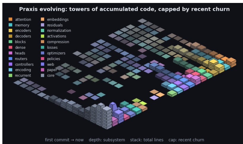
Figure 4: Praxis’s git history as an isometric terrain over the last 2309 commits. Each cell is one subsystem in one time window: a stack of base blocks for its accumulated size (total lines, recency-weighted) topped by a vivid cap for that window’s line churn - the standing codebase carrying the recent activity. Both are weighted by recency (the kernel the model applies to a sequence, turned on the repository): recent windows stack tall with bright caps while history thins toward the always-present prior - the low valley we roll into. Color fades from each subsystem’s hue toward a neutral prior into the past, banded in phased strata over a non-linear timescale. It is the bias/variance geometry read along the frequency axis (see the project notes): loud recent corrections over the quiet, ever-present base. By recency-weighted churn the current center of gravity is core, web, paper. The framework charts the hand that builds it.
