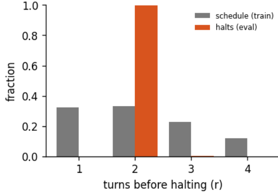
Figure 2: Halting distribution: the fraction of forward passes that stop after r turns, for the 4-turn recurrent loop of run calm-d-1, early-halt rate 50%, mean boundary KL 0.0532. schedule is the random loop-count the model trains under; halts is where the KL gate actually stops at inference. A mass pinned at the maximum (KL never collapsing) is the honest signature of a model that has not yet learned to converge early - the decision is real, not yet decisive.
