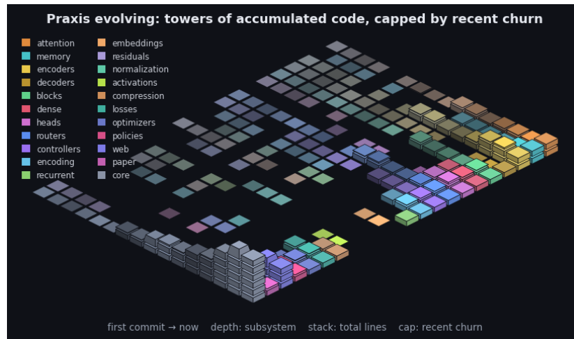
Figure 7: Praxis’s git history as an isometric terrain over the last 2214 commits. Each cell is one subsystem in one time window: a stack of base blocks for its accumulated size (total lines, recency-weighted) topped by a vivid cap for that window’s line churn - the standing codebase carrying the recent activity. Both are weighted by recency (the kernel the model applies to a sequence, turned on the repository): recent windows stack tall with bright caps while history thins toward the always-present prior - the low valley we roll into. Color fades from each subsystem’s hue toward a neutral prior into the past, banded in phased strata over a non-linear timescale. It is the bias/variance geometry read along the frequency axis (see the project notes): loud recent corrections over the quiet, ever-present base. By recency-weighted churn the current center of gravity is core, web, encoders. The framework charts the hand that builds it.
