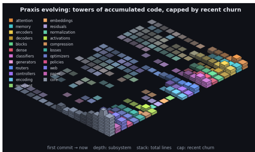
Figure 13: Praxis’s git history as an isometric terrain over the last 2645 commits. Each cell is one subsystem in one time window: a stack of base blocks for its accumulated size (total lines, recency-weighted) topped by a vivid cap for that window’s line churn - the standing codebase carrying the recent activity. Both are weighted by recency (the kernel the model applies to a sequence, turned on the repository): recent windows stack tall with bright caps while history thins toward the always-present prior - the low valley we roll into. Color fades from each subsystem’s hue toward a neutral prior into the past, banded in phased strata over a non-linear timescale. It is the bias/variance geometry read along the frequency axis (see the project notes): loud recent corrections over the quiet, ever-present base. By recency-weighted churn the current center of gravity is core, web, encoders. The framework charts the hand that builds it.
