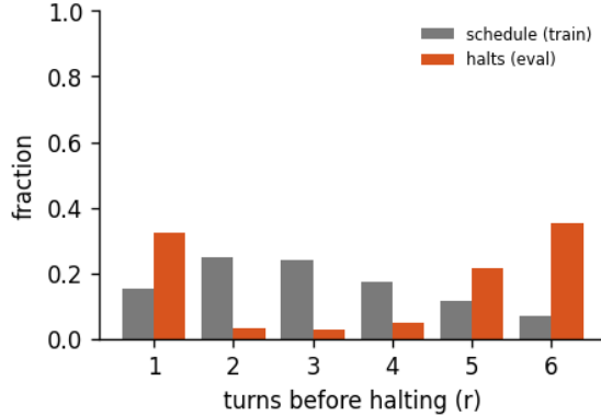
Figure 9: Halting distribution: the fraction of forward passes that stop after r turns, for the 6-turn recurrent loop of run byte-latent-a, early-halt rate 19%, mean boundary KL 0.0177. schedule is the random loop-count the model trains under; halts is where the KL gate actually stops at inference. A mass pinned at the maximum (KL never collapsing) is the honest signature of a model that has not yet learned to converge early - the decision is real, not yet decisive.
