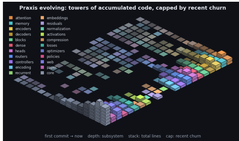
Figure 12: Praxis's git history as an isometric terrain over the last 2612 commits. Each cell is one subsystem in one time window: a stack of base blocks for its accumulated size (total lines, recency-weighted) topped by a vivid cap for that window's line churn - the standing codebase carrying the recent activity. Both are weighted by recency (the kernel the model applies to a sequence, turned on the repository): recent windows stack tall with bright caps while history thins toward the always-present prior - the low valley we roll into. Color fades from each subsystem's hue toward a neutral prior into the past, banded in phased strata over a non-linear timescale. It is the bias/variance geometry read along the frequency axis (see the project notes): loud recent corrections over the quiet, ever-present base. By recency-weighted churn the current center of gravity is core, web, encoders. The framework charts the hand that builds it.
