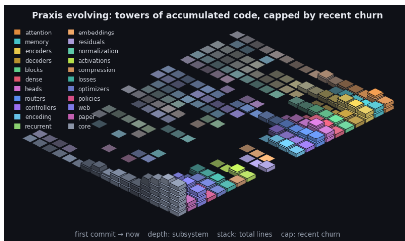
Figure 13: Praxis’s git history as an isometric terrain over the last 2564 commits. Each cell is one subsystem in one time window: a stack of base blocks for its accumulated size (total lines, recency-weighted) topped by a vivid cap for that window’s line churn - the standing codebase carrying the recent activity. Both are weighted by recency (the kernel the model applies to a sequence, turned on the repository): recent windows stack tall with bright caps while history thins toward the always-present prior - the low valley we roll into. Color fades from each subsystem’s hue toward a neutral prior into the past, banded in phased strata over a non-linear timescale. It is the bias/variance geometry read along the frequency axis (see the project notes): loud recent corrections over the quiet, ever-present base. By recency-weighted churn the current center of gravity is core, web, paper. The framework charts the hand that builds it.
