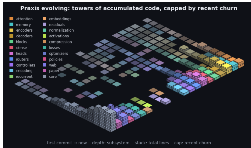
Figure 12: Praxis’s git history as an isometric terrain over the last 2493 commits. Each cell is one subsystem in one time window: a stack of base blocks for its accumulated size (total lines, recency-weighted) topped by a vivid cap for that window’s line churn - the standing codebase carrying the recent activity. Both are weighted by recency (the kernel the model applies to a sequence, turned on the repository): recent windows stack tall with bright caps while history thins toward the always-present prior - the low valley we roll into. Color fades from each subsystem’s hue toward a neutral prior into the past, banded in phased strata over a non-linear timescale. It is the bias/variance geometry read along the frequency axis (see the project notes): loud recent corrections over the quiet, ever-present base. By recency-weighted churn the current center of gravity is core, web, paper. The framework charts the hand that builds it.
