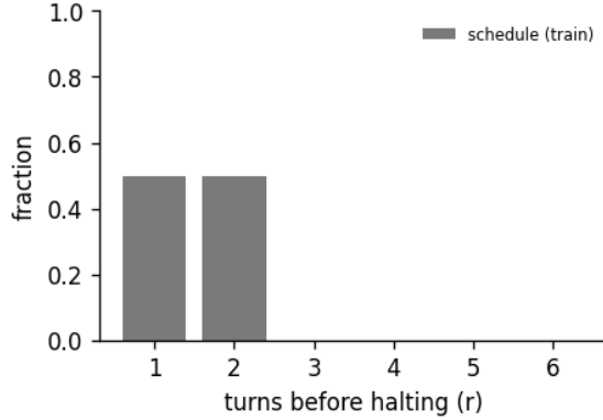
Figure 8: Halting distribution: the fraction of forward passes that stop after r turns, for the 6-turn recurrent loop of run abstractinator-j. schedule is the random loop-count the model trains under; halts is where the KL gate actually stops at inference. A mass pinned at the maximum (KL never collapsing) is the honest signature of a model that has not yet learned to converge early - the decision is real, not yet decisive.
