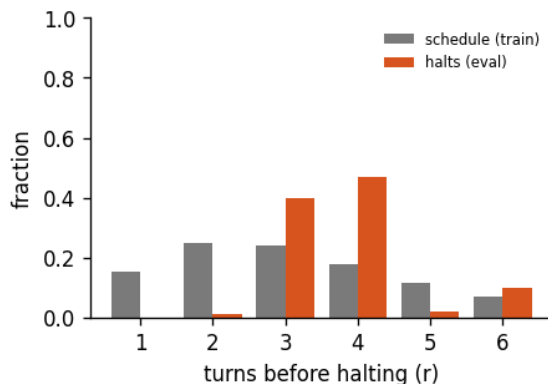
Figure 8: Halting distribution: the fraction of forward passes that stop after r turns, for the 6-turn recurrent loop of run abstractinator-w, early-halt rate 24%, mean boundary KL 0.123. schedule is the random loop-count the model trains under; halts is where the KL gate actually stops at inference. A mass pinned at the maximum (KL never collapsing) is the honest signature of a model that has not yet learned to converge early - the decision is real, not yet decisive.
