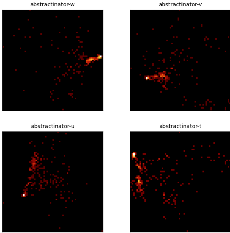
Figure 11: Center PCA density for the 4 most recent crystal-head runs ( abstractinator-w , abstractinator-v , abstractinator-u , abstractinator-t ). Each panel is the top-2 PCA projection of a head's vocabulary centers, binned to a 64 \times 64 density grid (log color) - the same snapshot the dashboard renders live. Different runs settle into structurally different geometries, not noise.
