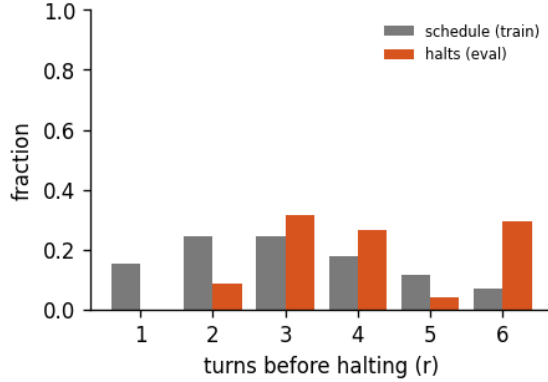
Figure 8: Halting distribution: the fraction of forward passes that stop after r turns, for the 6-turn recurrent loop of run abstractinator-h, early-halt rate 18%, mean boundary KL 0.293. schedule is the random loop-count the model trains under; halts is where the KL gate actually stops at inference. A mass pinned at the maximum (KL never collapsing) is the honest signature of a model that has not yet learned to converge early - the decision is real, not yet decisive.
