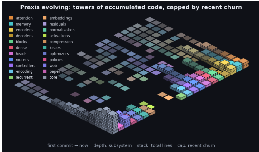
Figure 5: Praxis’s git history as an isometric terrain over the last 2232 commits. Each cell is one subsystem in one time window: a stack of base blocks for its accumulated size (total lines, recency-weighted) topped by a vivid cap for that window’s line churn - the standing codebase carrying the recent activity. Both are weighted by recency (the kernel the model applies to a sequence, turned on the repository): recent windows stack tall with bright caps while history thins toward the always-present prior - the low valley we roll into. Color fades from each subsystem’s hue toward a neutral prior into the past, banded in phased strata over a non-linear timescale. It is the bias/variance geometry read along the frequency axis (see the project notes): loud recent corrections over the quiet, ever-present base. By recency-weighted churn the current center of gravity is core, web, encoders. The framework charts the hand that builds it.
