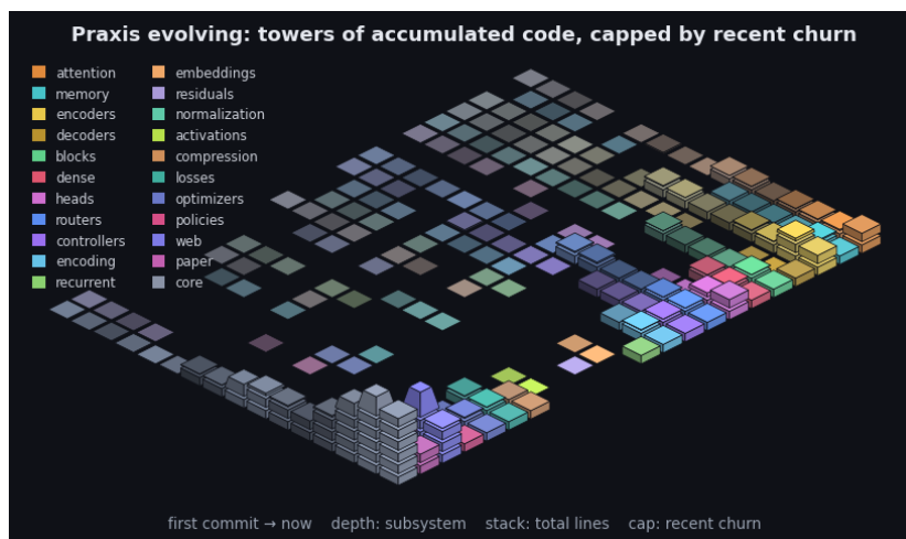
Figure 4: Praxis’s git history as an isometric terrain over the last 2308 commits. Each cell is one subsystem in one time window: a stack of base blocks for its accumulated size (total lines, recency-weighted) topped by a vivid cap for that window’s line churn - the standing codebase carrying the recent activity. Both are weighted by recency (the kernel the model applies to a sequence, turned on the repository): recent windows stack tall with bright caps while history thins toward the always-present prior - the low valley we roll into. Color fades from each subsystem’s hue toward a neutral prior into the past, banded in phased strata over a non-linear timescale. It is the bias/variance geometry read along the frequency axis (see the project notes): loud recent corrections over the quiet, ever-present base. By recency-weighted churn the current center of gravity is core, web, paper. The framework charts the hand that builds it.
