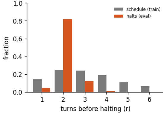
Figure 9: Halting distribution: the fraction of forward passes that stop after r turns, for the 6-turn recurrent loop of run byte-latent-a, early-halt rate 48%, mean boundary KL 0.0223. schedule is the random loop-count the model trains under; halts is where the KL gate actually stops at inference. A mass pinned at the maximum (KL never collapsing) is the honest signature of a model that has not yet learned to converge early - the decision is real, not yet decisive.
