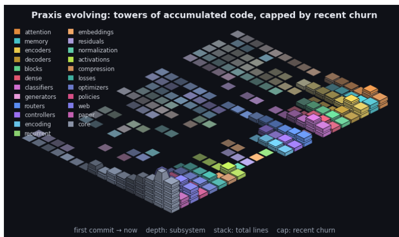
Figure 13: Praxis’s git history as an isometric terrain over the last 2659 commits. Each cell is one subsystem in one time window: a stack of base blocks for its accumulated size (total lines, recency-weighted) topped by a vivid cap for that window’s line churn - the standing codebase carrying the recent activity. Both are weighted by recency (the kernel the model applies to a sequence, turned on the repository): recent windows stack tall with bright caps while history thins toward the always-present prior - the low valley we roll into. Color fades from each subsystem’s hue toward a neutral prior into the past, banded in phased strata over a non-linear timescale. It is the bias/variance geometry read along the frequency axis (see the project notes): loud recent corrections over the quiet, ever-present base. By recency-weighted churn the current center of gravity is core, web, encoders. The framework charts the hand that builds it.
