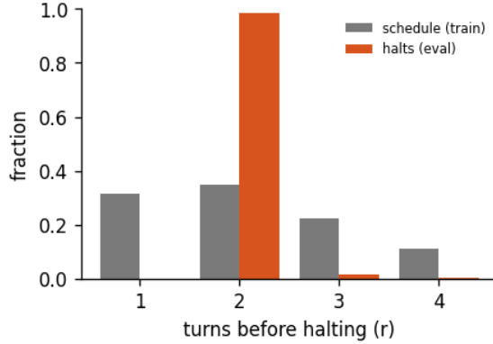
Figure 8: Halting distribution: the fraction of forward passes that stop after r turns, for the 4-turn recurrent loop of run abstractinator-g, early-halt rate 50%, mean boundary KL 0.238. schedule is the random loop-count the model trains under; halts is where the KL gate actually stops at inference. A mass pinned at the maximum (KL never collapsing) is the honest signature of a model that has not yet learned to converge early - the decision is real, not yet decisive.
