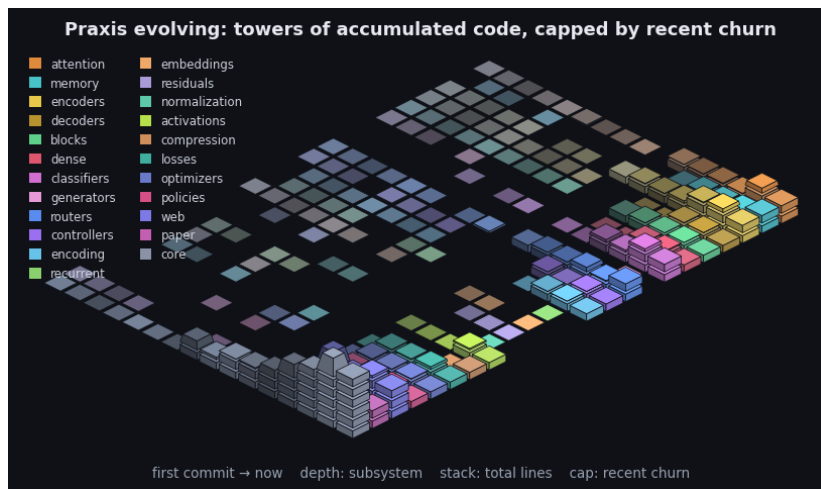
Figure 9: Praxis’s git history as an isometric terrain over the last 2696 commits. Each cell is one subsystem in one time window: a stack of base blocks for its accumulated size (total lines, recency-weighted) topped by a vivid cap for that window’s line churn - the standing codebase carrying the recent activity. Both are weighted by recency (the kernel the model applies to a sequence, turned on the repository): recent windows stack tall with bright caps while history thins toward the always-present prior - the low valley we roll into. Color fades from each subsystem’s hue toward a neutral prior into the past, banded in phased strata over a non-linear timescale. It is the bias/variance geometry read along the frequency axis (see the project notes): loud recent corrections over the quiet, ever-present base. By recency-weighted churn the current center of gravity is core, web, encoders. The framework charts the hand that builds it.
