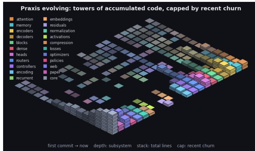
Figure 11: Praxis’s git history as an isometric terrain over the last 2433 commits. Each cell is one subsystem in one time window: a stack of base blocks for its accumulated size (total lines, recency-weighted) topped by a vivid cap for that window’s line churn - the standing codebase carrying the recent activity. Both are weighted by recency (the kernel the model applies to a sequence, turned on the repository): recent windows stack tall with bright caps while history thins toward the always-present prior - the low valley we roll into. Color fades from each subsystem’s hue toward a neutral prior into the past, banded in phased strata over a non-linear timescale. It is the bias/variance geometry read along the frequency axis (see the project notes): loud recent corrections over the quiet, ever-present base. By recency-weighted churn the current center of gravity is core, web, paper. The framework charts the hand that builds it.
