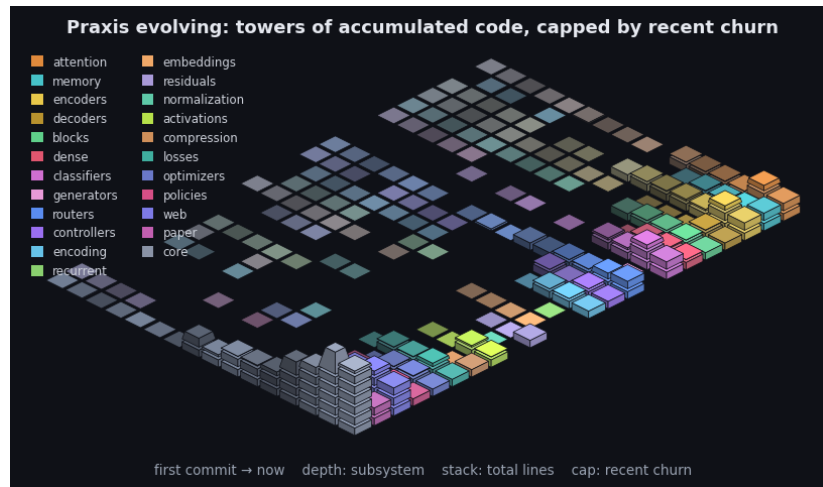
Figure 9: Praxis’s git history as an isometric terrain over the last 2621 commits. Each cell is one subsystem in one time window: a stack of base blocks for its accumulated size (total lines, recency-weighted) topped by a vivid cap for that window’s line churn - the standing codebase carrying the recent activity. Both are weighted by recency (the kernel the model applies to a sequence, turned on the repository): recent windows stack tall with bright caps while history thins toward the always-present prior - the low valley we roll into. Color fades from each subsystem’s hue toward a neutral prior into the past, banded in phased strata over a non-linear timescale. It is the bias/variance geometry read along the frequency axis (see the project notes): loud recent corrections over the quiet, ever-present base. By recency-weighted churn the current center of gravity is core, web, encoders. The framework charts the hand that builds it.
