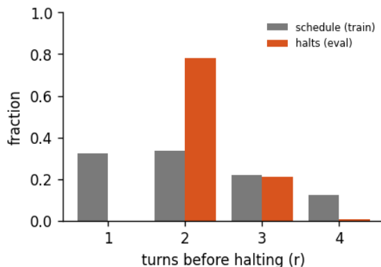
Figure 8: Halting distribution: the fraction of forward passes that stop after r turns, for the 4-turn recurrent loop of run abstractinator-f, early-halt rate 45%, mean boundary KL 0.425. schedule is the random loop-count the model trains under; halts is where the KL gate actually stops at inference. A mass pinned at the maximum (KL never collapsing) is the honest signature of a model that has not yet learned to converge early - the decision is real, not yet decisive.
