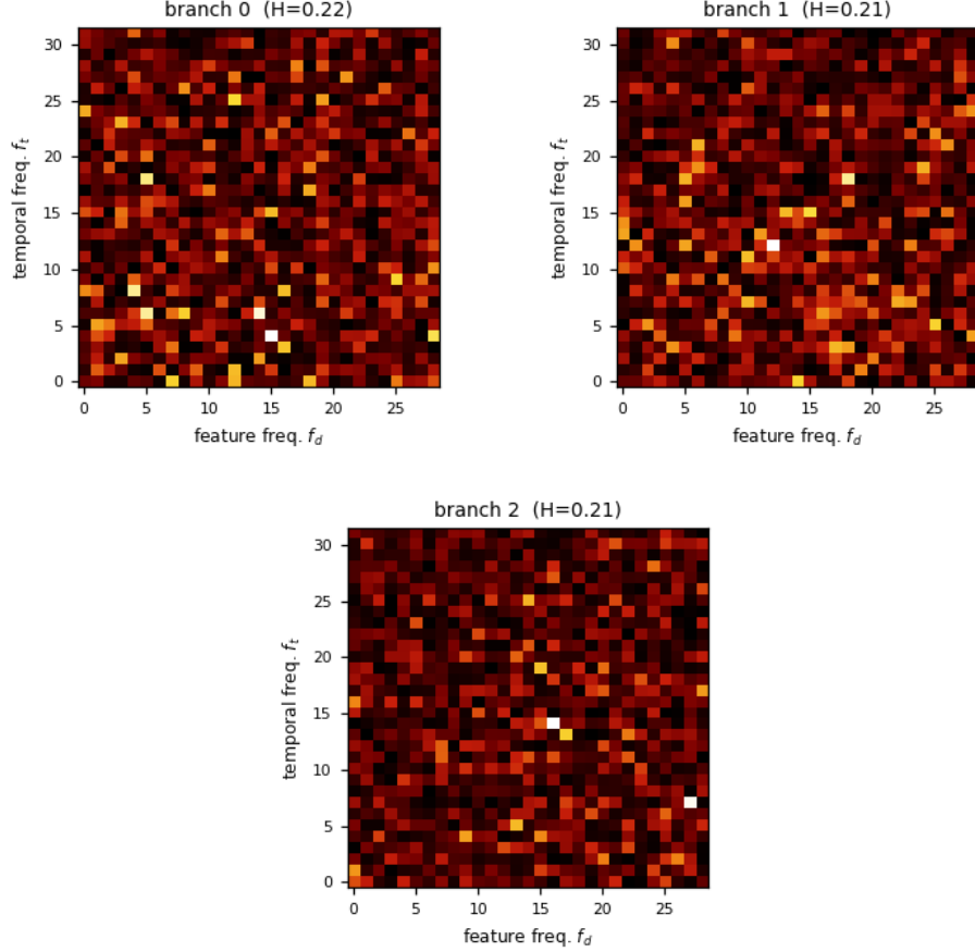
Figure 2: The static amplitude spectrum |a[f_t, f_d]| across the 3 arms of abstractinator-g’s prismatic head - the learned grid that, inverse-transformed through the frozen Weyl phases, becomes the bias field. This is the heatmap the text describes: energy that settles into a low-frequency band (small f_t, f_d ) is the corpus rhythm crystallizing, while a grid that stays uniform is a field still indistinguishable from noise. Hoyer concentrations H = 0.22, 0.21, 0.21 (left to right) quantifies it on the same [0, 1] scale the prose names (1 = a single cell, 0 = uniform), computed from this very tensor by concentration() - the same value the dashboard logs live. The pink 1/f^\alpha prior lives in the frozen basis, not in these amplitudes, so the grid shown is exactly what the head exposes.
