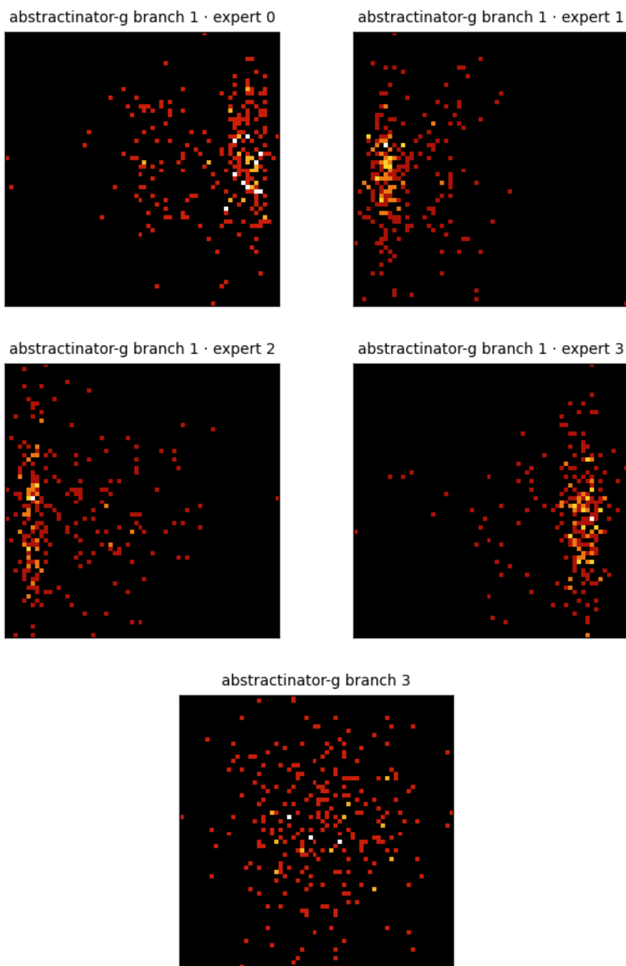
Figure 11: Center PCA density for the 5 crystal heads of abstractinator-g - a single multi-head model (prismatic4’s VEAR crystal bank), so these are that run’s own heads (branch 1 · expert 0, branch 1 · expert 1, branch 1 · expert 2, branch 1 · expert 3, branch 3), not a cross-run mix. Each panel is the top-2 PCA projection of a head’s vocabulary centers, binned to a 64×64 density grid (log color) - the same snapshot the dashboard renders live. The bank’s experts settle into structurally distinct geometries - the between-expert variance the router selects over.
