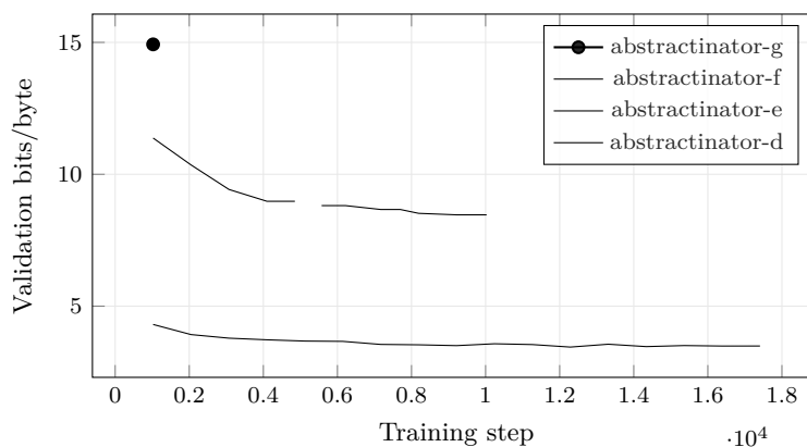
Figure 13: Bits per Byte across the 4 most recent experiments with comparable validation curves; the leading run (abstractinator-g) is drawn in bold. Generated from run logs - metrics that are not comparable across families (token loss vs. byte bits-per-byte vs. codec/CALM BrierLM) are excluded by construction, so the curves on this axis mean the same thing.
