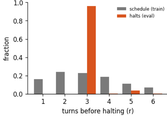
Figure 8: Halting distribution: the fraction of forward passes that stop after r turns, for the 6-turn recurrent loop of run abstractinator-m, early-halt rate 32%, mean boundary KL 0.462. schedule is the random loop-count the model trains under; halts is where the KL gate actually stops at inference. A mass pinned at the maximum (KL never collapsing) is the honest signature of a model that has not yet learned to converge early - the decision is real, not yet decisive.
