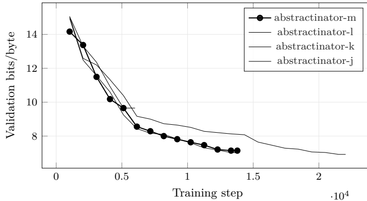
Figure 13: Bits per Byte across the 4 most recent experiments with comparable validation curves; the current experiment ( abstractinator-m ) is drawn in bold. Bold marks which run this build is reporting on , not which run scores best. The curves end wherever each run stopped, so they are at different points along their own training, and their endpoints are not a ranking. Generated from run logs - metrics that are not comparable across families (token loss vs. byte bits-per-byte vs. codec/CALM BrierLM) are excluded by construction, so the curves on this axis mean the same thing.
