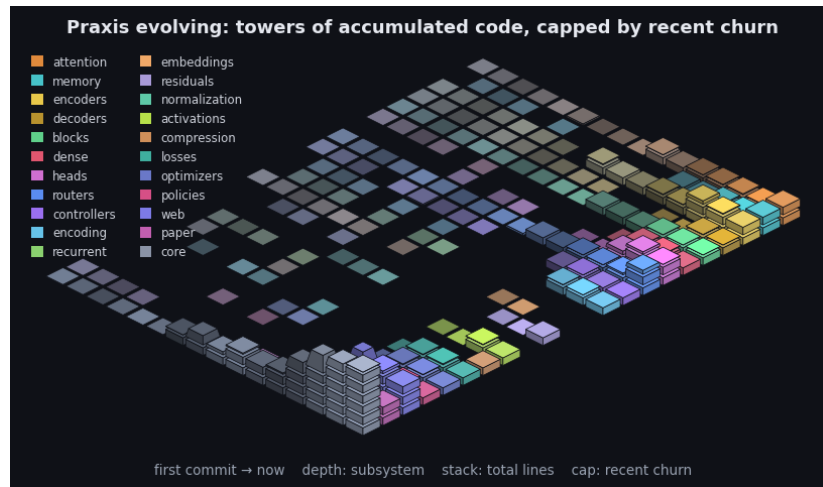
Figure 12: Praxis’s git history as an isometric terrain over the last 2508 commits. Each cell is one subsystem in one time window: a stack of base blocks for its accumulated size (total lines, recency-weighted) topped by a vivid cap for that window’s line churn - the standing codebase carrying the recent activity. Both are weighted by recency (the kernel the model applies to a sequence, turned on the repository): recent windows stack tall with bright caps while history thins toward the always-present prior - the low valley we roll into. Color fades from each subsystem’s hue toward a neutral prior into the past, banded in phased strata over a non-linear timescale. It is the bias/variance geometry read along the frequency axis (see the project notes): loud recent corrections over the quiet, ever-present base. By recency-weighted churn the current center of gravity is core, web, paper. The framework charts the hand that builds it.
