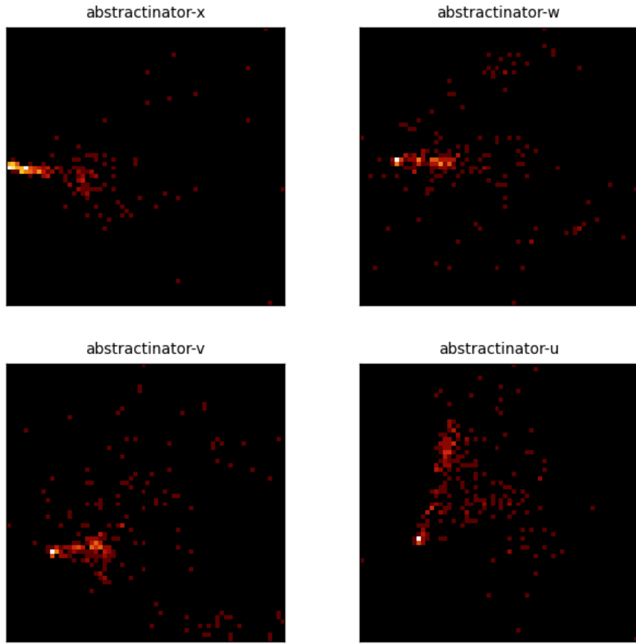
Figure 11: Center PCA density for the 4 most recent crystal-head runs (abstractinator-x, abstractinator-w, abstractinator-v, abstractinator-u). Each panel is the top-2 PCA projection of a head’s vocabulary centers, binned to a 64 \times 64 density grid (log color) - the same snapshot the dashboard renders live. Different runs settle into structurally different geometries, not noise.
