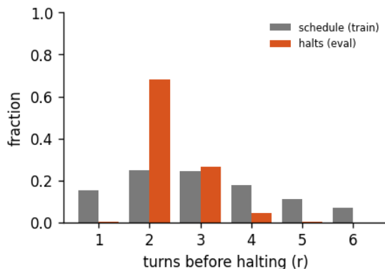
Figure 8: Halting distribution: the fraction of forward passes that stop after r turns, for the 6-turn recurrent loop of run abstractinator-x, early-halt rate 42%, mean boundary KL 0.808. schedule is the random loop-count the model trains under; halts is where the KL gate actually stops at inference. A mass pinned at the maximum (KL never collapsing) is the honest signature of a model that has not yet learned to converge early - the decision is real, not yet decisive.
