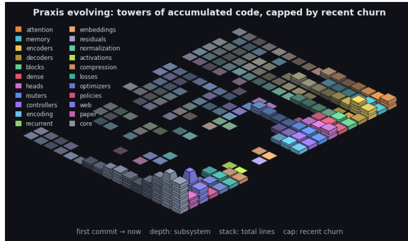
Figure 5: Praxis’s git history as an isometric terrain over the last 2355 commits. Each cell is one subsystem in one time window: a stack of base blocks for its accumulated size (total lines, recency-weighted) topped by a vivid cap for that window’s line churn - the standing codebase carrying the recent activity. Both are weighted by recency (the kernel the model applies to a sequence, turned on the repository): recent windows stack tall with bright caps while history thins toward the always-present prior - the low valley we roll into. Color fades from each subsystem’s hue toward a neutral prior into the past, banded in phased strata over a non-linear timescale. It is the bias/variance geometry read along the frequency axis (see the project notes): loud recent corrections over the quiet, ever-present base. By recency-weighted churn the current center of gravity is core, web, paper. The framework charts the hand that builds it.
