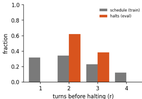
Figure 2: Halting distribution: the fraction of forward passes that stop after r turns, for the 4-turn recurrent loop of run calm-d-1, early-halt rate 42%, mean boundary KL 0.0942. schedule is the random loop-count the model trains under; halts is where the KL gate actually stops at inference. A mass pinned at the maximum (KL never collapsing) is the honest signature of a model that has not yet learned to converge early - the decision is real, not yet decisive.
