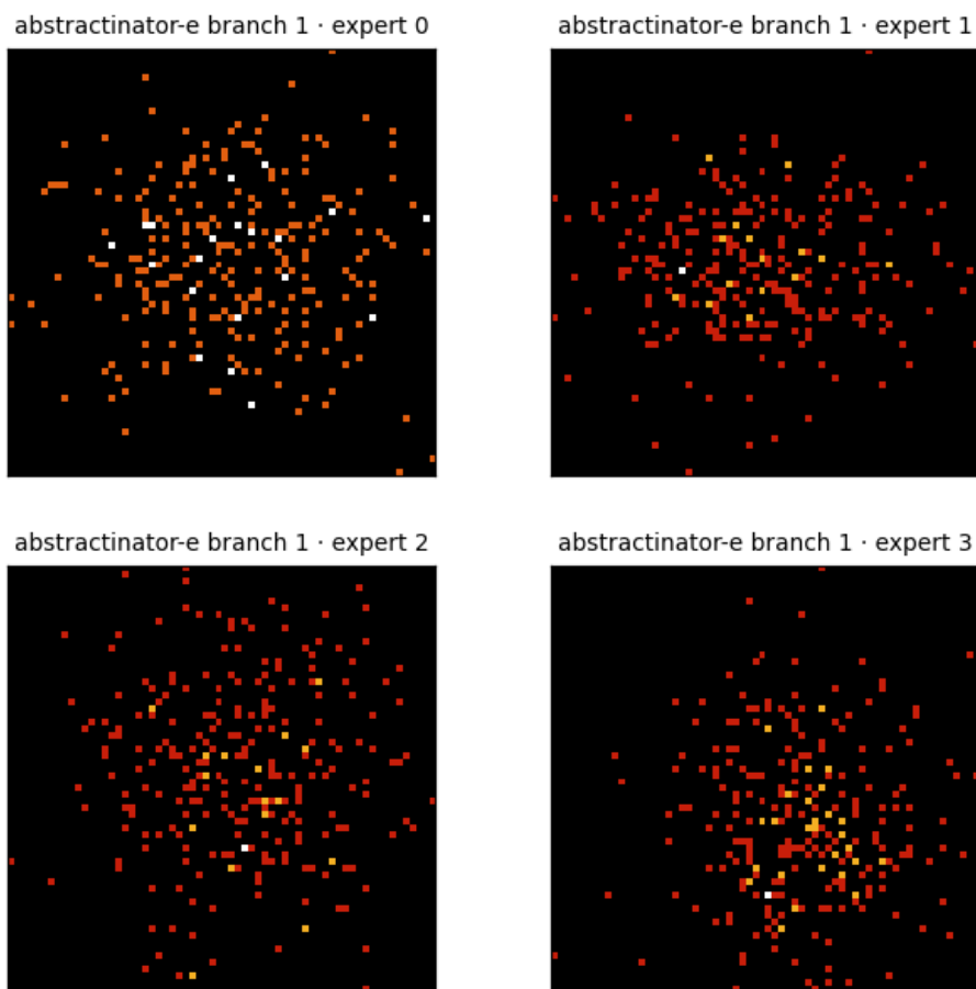
Figure 11: Center PCA density for the 4 crystal heads of abstractinator-e - a single multi-head model (prismatic4’s VEAR crystal bank), so these are that run’s own heads (branch 1 · expert 0, branch 1 · expert 1, branch 1 · expert 2, branch 1 · expert 3), not a cross-run mix. Each panel is the top-2 PCA projection of a head’s vocabulary centers, binned to a 64 \times 64 density grid (log color) - the same snapshot the dashboard renders live. The bank’s experts settle into structurally distinct geometries - the between-expert variance the router selects over.
