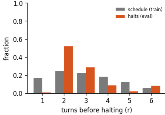
Figure 9: Halting distribution: the fraction of forward passes that stop after r turns, for the 6-turn recurrent loop of run abstractinator-r, early-halt rate 33%, mean boundary KL 0.272. schedule is the random loop-count the model trains under; halts is where the KL gate actually stops at inference. A mass pinned at the maximum (KL never collapsing) is the honest signature of a model that has not yet learned to converge early - the decision is real, not yet decisive.
