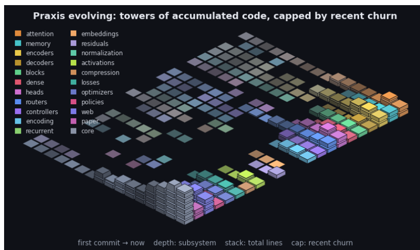
Figure 13: Praxis’s git history as an isometric terrain over the last 2587 commits. Each cell is one subsystem in one time window: a stack of base blocks for its accumulated size (total lines, recency-weighted) topped by a vivid cap for that window’s line churn - the standing codebase carrying the recent activity. Both are weighted by recency (the kernel the model applies to a sequence, turned on the repository): recent windows stack tall with bright caps while history thins toward the always-present prior - the low valley we roll into. Color fades from each subsystem’s hue toward a neutral prior into the past, banded in phased strata over a non-linear timescale. It is the bias/variance geometry read along the frequency axis (see the project notes): loud recent corrections over the quiet, ever-present base. By recency-weighted churn the current center of gravity is core, web, paper. The framework charts the hand that builds it.
