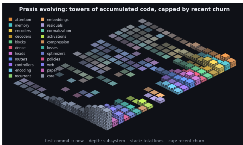
Figure 13: Praxis’s git history as an isometric terrain over the last 2561 commits. Each cell is one subsystem in one time window: a stack of base blocks for its accumulated size (total lines, recency-weighted) topped by a vivid cap for that window’s line churn - the standing codebase carrying the recent activity. Both are weighted by recency (the kernel the model applies to a sequence, turned on the repository): recent windows stack tall with bright caps while history thins toward the always-present prior - the low valley we roll into. Color fades from each subsystem’s hue toward a neutral prior into the past, banded in phased strata over a non-linear timescale. It is the bias/variance geometry read along the frequency axis (see the project notes): loud recent corrections over the quiet, ever-present base. By recency-weighted churn the current center of gravity is core, web, paper. The framework charts the hand that builds it.
