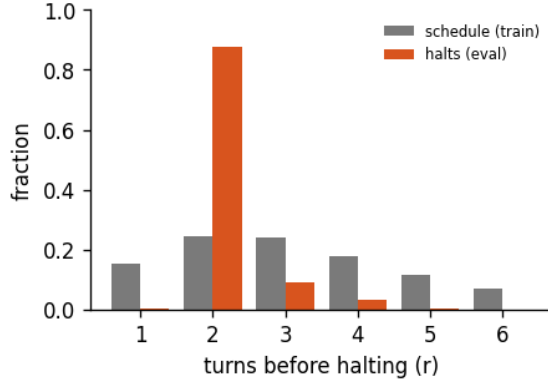
Figure 8: Halting distribution: the fraction of forward passes that stop after r turns, for the 6-turn recurrent loop of run abstractinator-e, early-halt rate 46%, mean boundary KL 0.775. schedule is the random loop-count the model trains under; halts is where the KL gate actually stops at inference. A mass pinned at the maximum (KL never collapsing) is the honest signature of a model that has not yet learned to converge early - the decision is real, not yet decisive.
