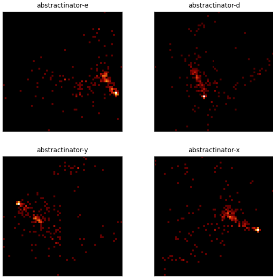
Figure 11: Center PCA density for the 4 most recent crystal-head runs ( abstractinator-e , abstractinator-d , abstractinator-y , abstractinator-x ). Each panel is the top-2 PCA projection of a head's vocabulary centers, binned to a 64 \times 64 density grid (log color) - the same snapshot the dashboard renders live. Different runs settle into structurally different geometries, not noise.
