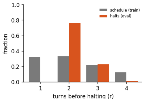
Figure 8: Halting distribution: the fraction of forward passes that stop after r turns, for the 4-turn recurrent loop of run abstractinator-f, early-halt rate 44%, mean boundary KL 0.411. schedule is the random loop-count the model trains under; halts is where the KL gate actually stops at inference. A mass pinned at the maximum (KL never collapsing) is the honest signature of a model that has not yet learned to converge early - the decision is real, not yet decisive.
