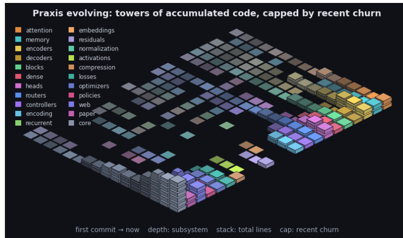
Figure 12: Praxis’s git history as an isometric terrain over the last 2446 commits. Each cell is one subsystem in one time window: a stack of base blocks for its accumulated size (total lines, recency-weighted) topped by a vivid cap for that window’s line churn - the standing codebase carrying the recent activity. Both are weighted by recency (the kernel the model applies to a sequence, turned on the repository): recent windows stack tall with bright caps while history thins toward the always-present prior - the low valley we roll into. Color fades from each subsystem’s hue toward a neutral prior into the past, banded in phased strata over a non-linear timescale. It is the bias/variance geometry read along the frequency axis (see the project notes): loud recent corrections over the quiet, ever-present base. By recency-weighted churn the current center of gravity is core, web, paper. The framework charts the hand that builds it.
