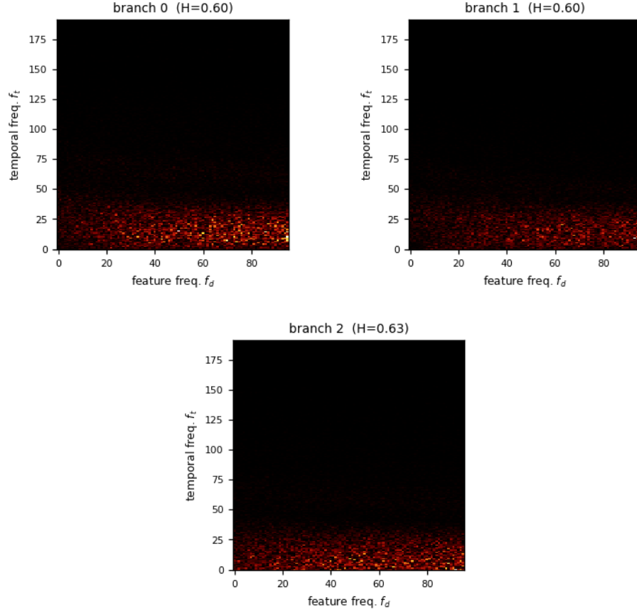
Figure 2: The static amplitude spectrum |a[f_t, f_d]| across the 3 arms of abstractinator-b’s prismatic head - the learned grid that, inverse-transformed through the frozen Weyl phases, becomes the bias field. This is the heatmap the text describes: energy that settles into a low-frequency band (small f_t, f_d ) is the corpus rhythm crystallizing, while a grid that stays uniform is a field still indistinguishable from noise. Hoyer concentrations H = 0.60, 0.60, 0.63 (left to right) quantifies it on the same [0, 1] scale the prose names (1 = a single cell, 0 = uniform), computed from this very tensor by concentration() - the same value the dashboard logs live. The pink 1/f^\alpha prior lives in the frozen basis, not in these amplitudes, so the grid shown is exactly what the head exposes.
