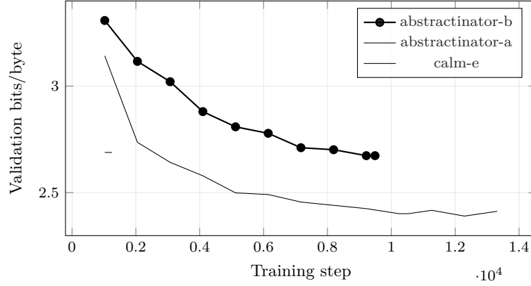
Figure 11: Bits per Byte across the 3 most recent experiments with comparable validation curves; the leading run (abstractinator-b) is drawn in bold. Generated from run logs - metrics that are not comparable across families (token loss vs. byte bits-per-byte vs. codec/CALM BrierLM) are excluded by construction, so the curves on this axis mean the same thing.
