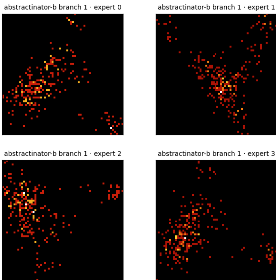
Figure 9: Center PCA density for the 4 crystal heads of abstractinator-b - a single multi-head model (prismatic4’s VEAR crystal bank), so these are that run’s own heads (branch 1 · expert 0, branch 1 · expert 1, branch 1 · expert 2, branch 1 · expert 3), not a cross-run mix. Each panel is the top-2 PCA projection of a head’s vocabulary centers, binned to a 64 \times 64 density grid (log color) - the same snapshot the dashboard renders live. The bank’s experts settle into structurally distinct geometries - the between-expert variance the router selects over.
