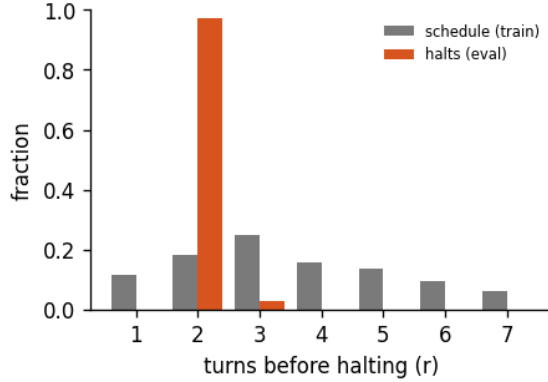
Figure 6: Halting distribution: the fraction of forward passes that stop after r turns, for the 7-turn recurrent loop of run abstractinator-b, early-halt rate 49%, mean boundary KL 0.352. schedule is the random loop-count the model trains under; halts is where the KL gate actually stops at inference. A mass pinned at the maximum (KL never collapsing) is the honest signature of a model that has not yet learned to converge early - the decision is real, not yet decisive.
