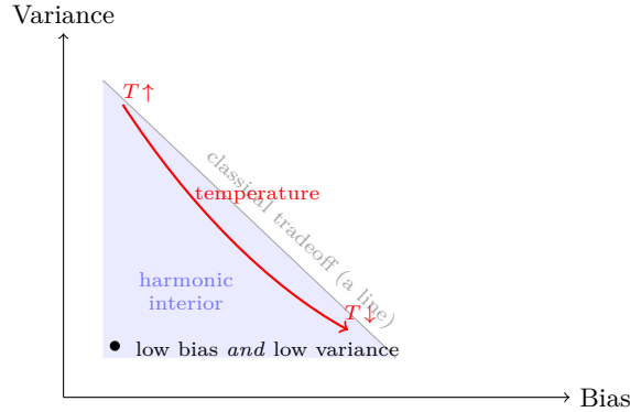
Figure 2: Bias and variance as orthogonal coordinates. Classically a model must sit somewhere on the gray line: less of one means more of the other. When a static spectrum supplies bias and an input-conditional modulation supplies variance, the two decouple, and the interior (shaded) becomes reachable - lower bias and lower variance than any point on the line. Temperature is a path through this space, not noise added at a fixed point.
