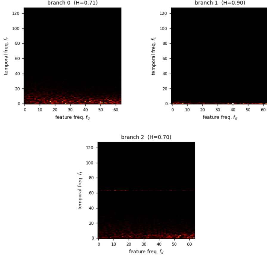
Figure 1: The static amplitude spectrum |a[f_t, f_d]| across the 3 arms of calm-d-1's prismatic head - the learned grid that, inverse-transformed through the frozen Weyl phases, becomes the bias field. This is the heatmap the text describes: energy that settles into a low-frequency band (small f_t, f_d ) is the corpus rhythm crystallizing, while a grid that stays uniform is a field still indistinguishable from noise. Hoyer concentrations H = 0.71, 0.90, 0.70 (left to right) quantifies it on the same [0, 1] scale the prose names (1 = a single cell, 0 = uniform), computed from this very tensor by concentration() - the same value the dashboard logs live. The pink 1/f^\alpha prior lives in the frozen basis, not in these amplitudes, so the grid shown is exactly what the head exposes.
