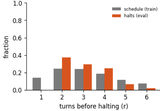
Figure 8: Halting distribution: the fraction of forward passes that stop after r turns, for the 6-turn recurrent loop of run abstractinator-g, early-halt rate 32%, mean boundary KL 0.269. schedule is the random loop-count the model trains under; halts is where the KL gate actually stops at inference. A mass pinned at the maximum (KL never collapsing) is the honest signature of a model that has not yet learned to converge early - the decision is real, not yet decisive.
