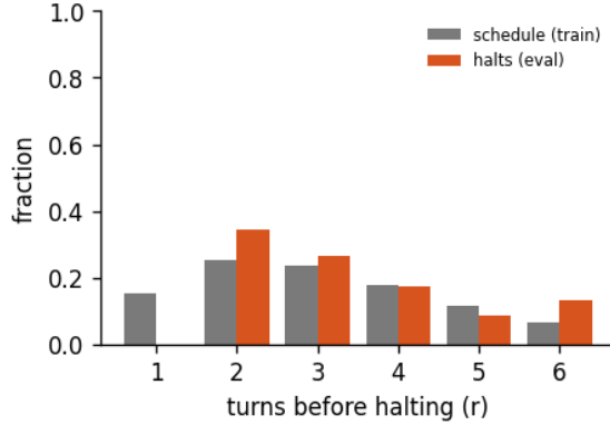
Figure 8: Halting distribution: the fraction of forward passes that stop after r turns, for the 6-turn recurrent loop of run abstractinator-q, early-halt rate 27%, mean boundary KL 0.392. schedule is the random loop-count the model trains under; halts is where the KL gate actually stops at inference. A mass pinned at the maximum (KL never collapsing) is the honest signature of a model that has not yet learned to converge early - the decision is real, not yet decisive.
