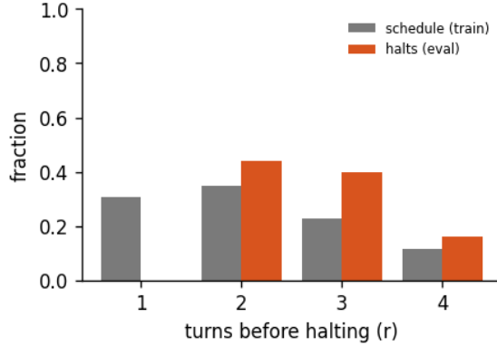
Figure 8: Halting distribution: the fraction of forward passes that stop after r turns, for the 4-turn recurrent loop of run abstractinator-g, early-halt rate 33%, mean boundary KL 0.264. schedule is the random loop-count the model trains under; halts is where the KL gate actually stops at inference. A mass pinned at the maximum (KL never collapsing) is the honest signature of a model that has not yet learned to converge early - the decision is real, not yet decisive.
