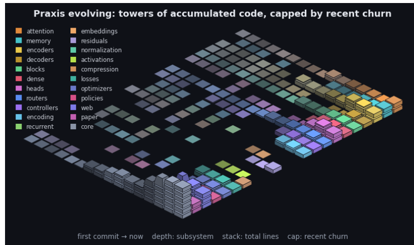
Figure 12: Praxis’s git history as an isometric terrain over the last 2461 commits. Each cell is one subsystem in one time window: a stack of base blocks for its accumulated size (total lines, recency-weighted) topped by a vivid cap for that window’s line churn - the standing codebase carrying the recent activity. Both are weighted by recency (the kernel the model applies to a sequence, turned on the repository): recent windows stack tall with bright caps while history thins toward the always-present prior - the low valley we roll into. Color fades from each subsystem’s hue toward a neutral prior into the past, banded in phased strata over a non-linear timescale. It is the bias/variance geometry read along the frequency axis (see the project notes): loud recent corrections over the quiet, ever-present base. By recency-weighted churn the current center of gravity is core, web, paper. The framework charts the hand that builds it.
