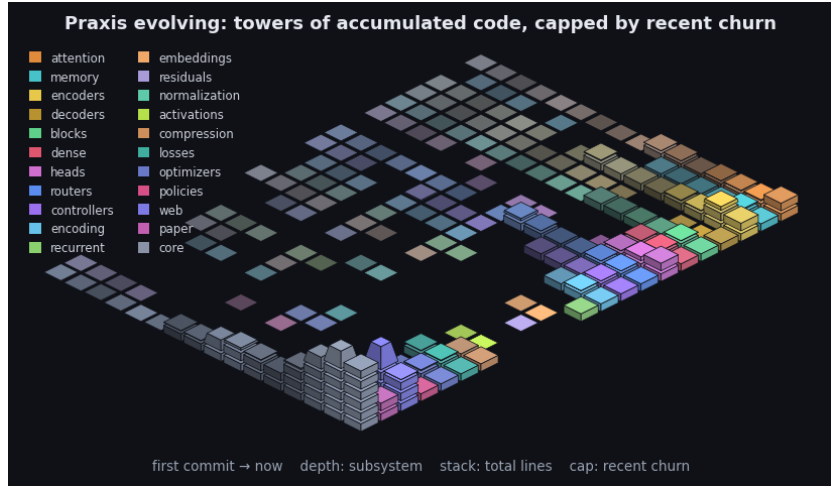
Figure 4: Praxis’s git history as an isometric terrain over the last 2336 commits. Each cell is one subsystem in one time window: a stack of base blocks for its accumulated size (total lines, recency-weighted) topped by a vivid cap for that window’s line churn - the standing codebase carrying the recent activity. Both are weighted by recency (the kernel the model applies to a sequence, turned on the repository): recent windows stack tall with bright caps while history thins toward the always-present prior - the low valley we roll into. Color fades from each subsystem’s hue toward a neutral prior into the past, banded in phased strata over a non-linear timescale. It is the bias/variance geometry read along the frequency axis (see the project notes): loud recent corrections over the quiet, ever-present base. By recency-weighted churn the current center of gravity is core, web, paper. The framework charts the hand that builds it.
