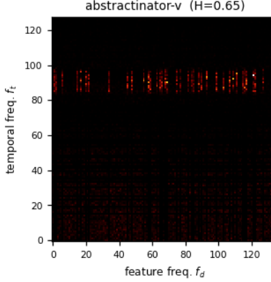
Figure 2: The static amplitude spectrum |a[f_t, f_d]| for abstractinator-v - the learned grid that, inverse-transformed through the frozen Weyl phases, becomes the bias field. This is the heatmap the text describes: energy that settles into a low-frequency band (small f_t, f_d ) is the corpus rhythm crystallizing, while a grid that stays uniform is a field still indistinguishable from noise. Hoyer concentration H = 0.65 quantifies it on the same [0, 1] scale the prose names (1 = a single cell, 0 = uniform), computed from this very tensor - the same value the dashboard logs live. The pink 1/f^\alpha prior lives in the frozen basis, not in these amplitudes, so the grid shown is exactly what the head exposes.
