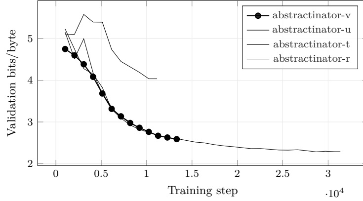
Figure 13: Bits per Byte across the 4 most recent experiments with comparable validation curves; the current experiment (abstractinator-v) is drawn in bold. Bold marks which run this build is reporting on , not which run scores best. The curves end wherever each run stopped, so they are at different points along their own training, and their endpoints are not a ranking. Generated from run logs - metrics that are not comparable across families (token loss vs. byte bits-per-byte vs. codec/CALM BrierLM) are excluded by construction, so the curves on this axis mean the same thing.
