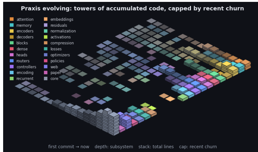
Figure 7: Praxis’s git history as an isometric terrain over the last 2226 commits. Each cell is one subsystem in one time window: a stack of base blocks for its accumulated size (total lines, recency-weighted) topped by a vivid cap for that window’s line churn - the standing codebase carrying the recent activity. Both are weighted by recency (the kernel the model applies to a sequence, turned on the repository): recent windows stack tall with bright caps while history thins toward the always-present prior - the low valley we roll into. Color fades from each subsystem’s hue toward a neutral prior into the past, banded in phased strata over a non-linear timescale. It is the bias/variance geometry read along the frequency axis (see the project notes): loud recent corrections over the quiet, ever-present base. By recency-weighted churn the current center of gravity is core, web, encoders. The framework charts the hand that builds it.
