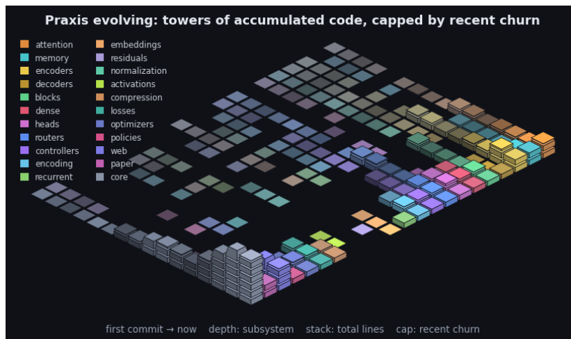
Figure 3: Praxis’s git history as an isometric terrain over the last 2265 commits. Each cell is one subsystem in one time window: a stack of base blocks for its accumulated size (total lines, recency-weighted) topped by a vivid cap for that window’s line churn - the standing codebase carrying the recent activity. Both are weighted by recency (the kernel the model applies to a sequence, turned on the repository): recent windows stack tall with bright caps while history thins toward the always-present prior - the low valley we roll into. Color fades from each subsystem’s hue toward a neutral prior into the past, banded in phased strata over a non-linear timescale. It is the bias/variance geometry read along the frequency axis (see the project notes): loud recent corrections over the quiet, ever-present base. By recency-weighted churn the current center of gravity is core, web, encoders. The framework charts the hand that builds it.
