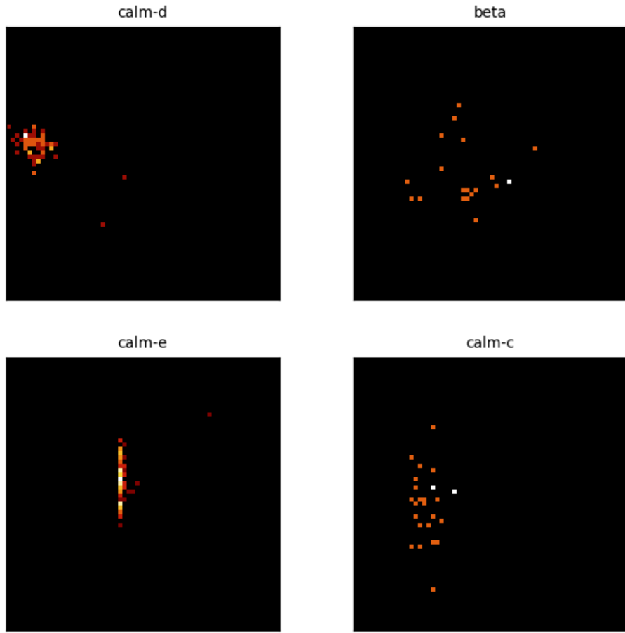
Figure 2: Center PCA density for the 4 most recent crystal-head runs (calm-d, beta, calm-e, calm-c). Each panel is the top-2 PCA projection of a head’s vocabulary centers, binned to a 64 \times 64 density grid (log color) - the same snapshot the dashboard renders live. Different runs settle into structurally different geometries, not noise.
